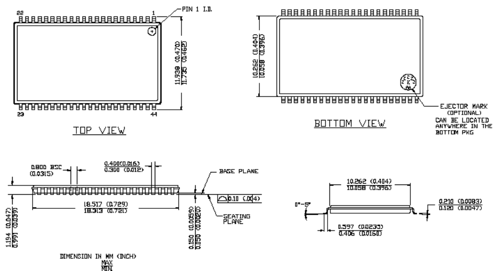
Figure 17. 44-Pin TSOP II (51-85087)
