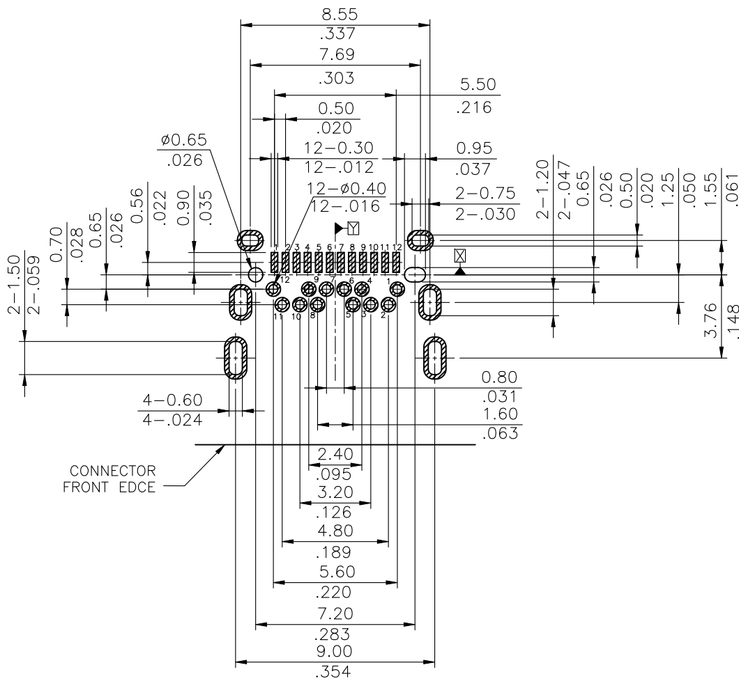
RECOMMENDED P.C.B. LAYOUT (T:1.00mm) TOLERANCE ±0.05mm
