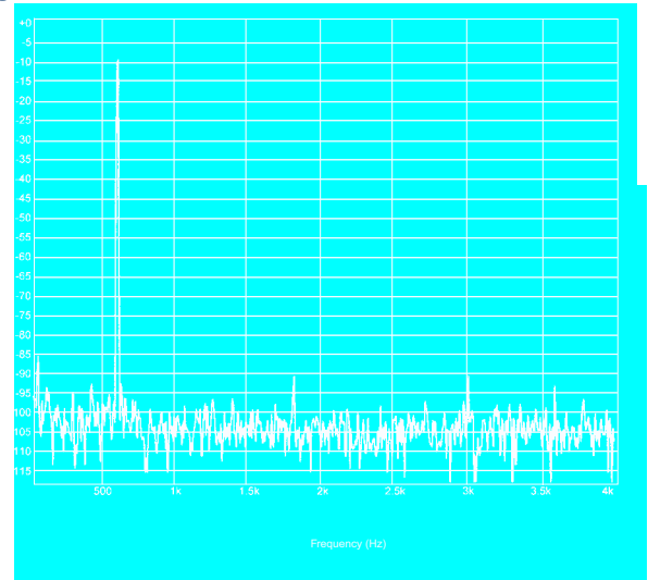
Figure 10. Receive THD on RX
