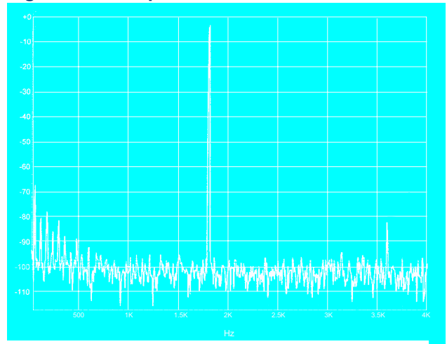
Figure 15. Snoop Circuit THD + N
