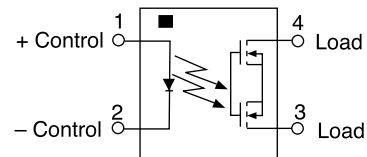
CPC1030N Pinout
