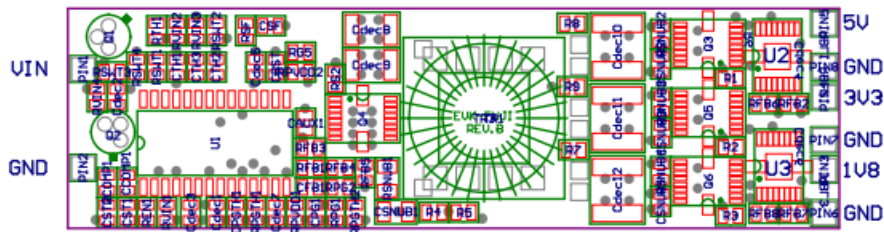
Figure 3: PCB layout (L=3''x L=1'')
