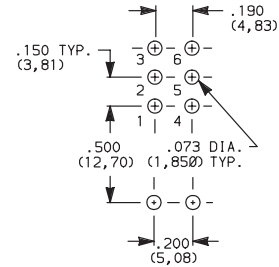
PC MOUNTING
