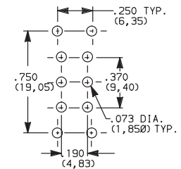
PC MOUNTING
