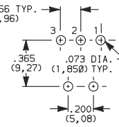
7101MD9A4BE Horizontal Actuation SPDT
