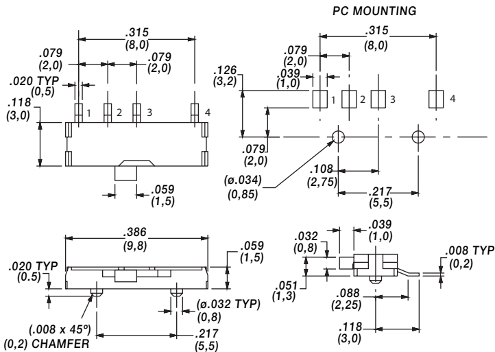
SWITCH SHOWN IN POSITION 1
