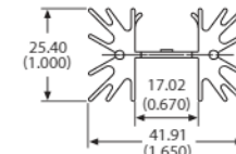
VIEW A-A SINGLE HEAT SINK DEVICE
