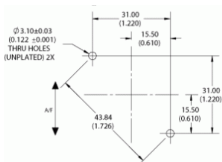
Mounting Details:
