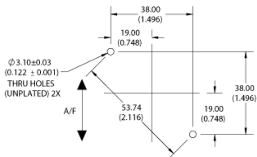
Mounting Details:
