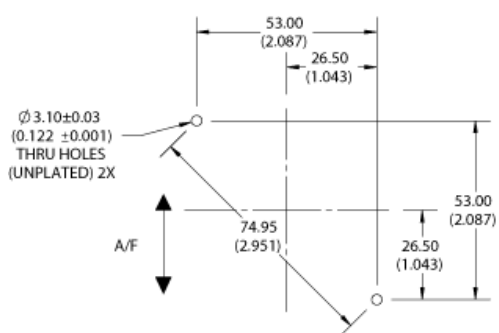
Mounting Details:
