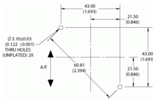
Mounting Details:
