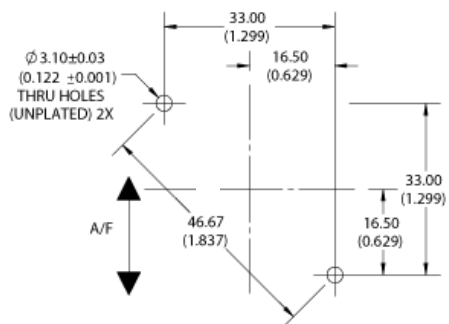
Mounting Details:
