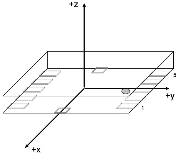
Figure 18: Axes orientation of the SMB380
