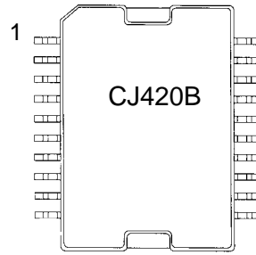
POWER-SO20
