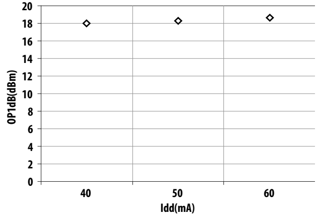
Figure 14. OP1dB vs I_{dd} at 5V Tuned for Optimum OIP3 and Fmin at 900MHz
