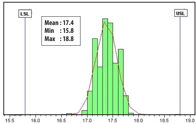
Figure 4. Gain @ 900MHz, 5V, 50mA Mean = 17.4
