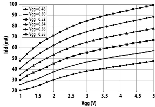
Figure 16. I-V curve
