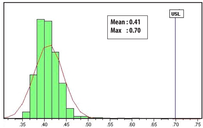
Figure 2. Noise Figure @ 900MHz, 5V, 50mA Mean = 0.41
