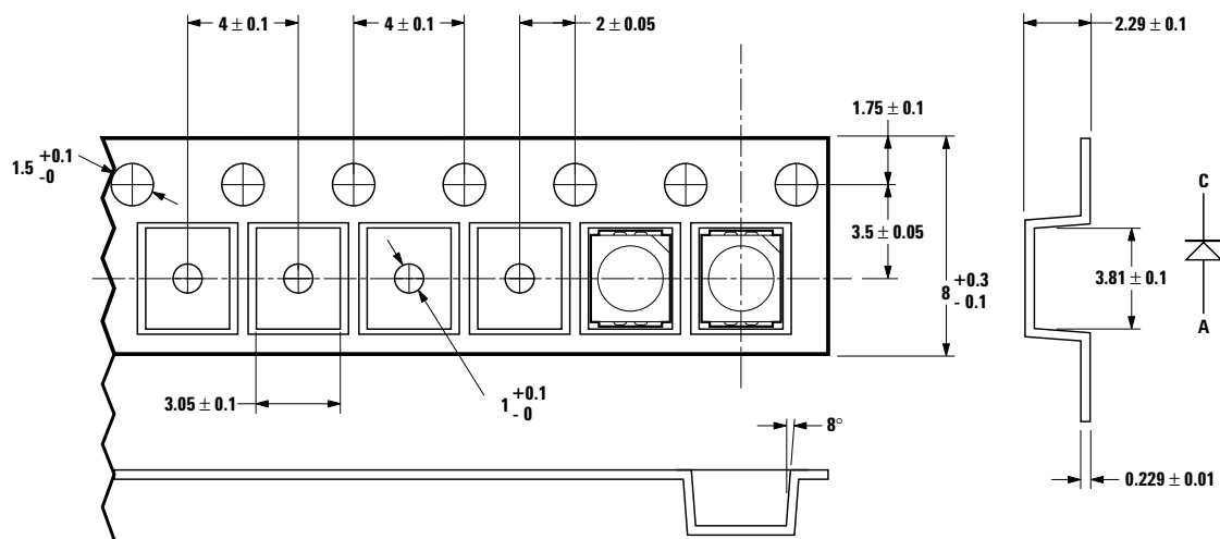
Figure 10. Tape dimension.
