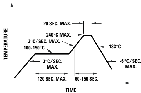
Figure 6a. Recommended SnPb reflow soldering profile.
