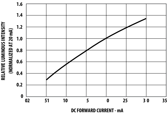
Figure 2. Relative intensity vs. forward current.
