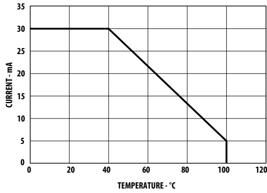
Figure 4. Maximum forward current vs. ambient temperature. Derated based on T J MAX = 110°C, Rθ JA = 500°C/W.
