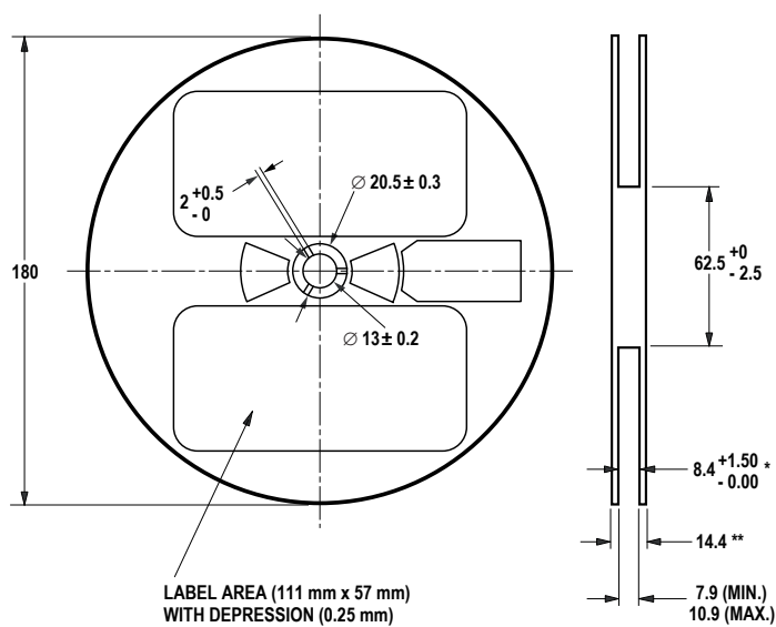
Figure 11. Reel dimensions.
