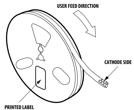
Figure 12. Reeling orientation.
