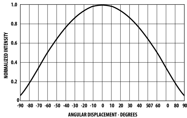
Figure 5. Radiation pattern.
