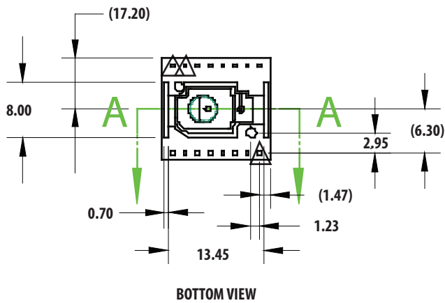
Figure 2. Package outline drawing
