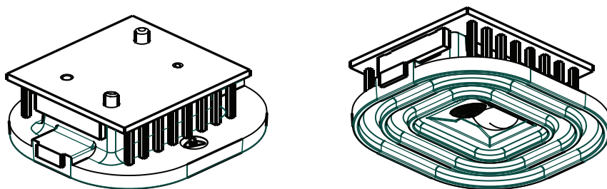
Figure 4. Isometric drawing of ADNS-9500 sensor and ADNS-6190-002 lens
