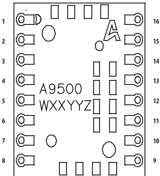
Figure 1. Package Pinout
