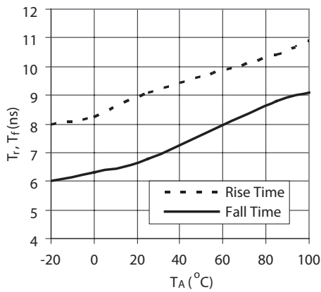
Figure 3. Typical rise and fall time vs temperature
