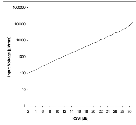
Figure 7. Sensitivity over RSSI
