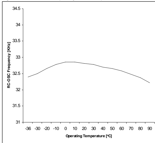
Figure 9. RC-Osc Frequency over Temperature (calibr.)
