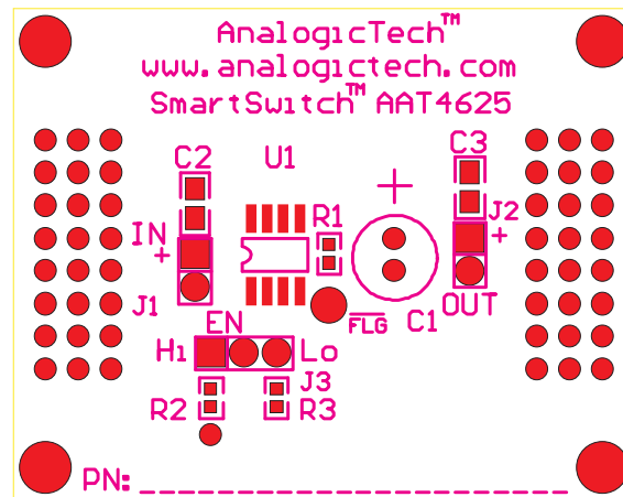
Figure 6: AAT4625 Evaluation Board Top Side Silk Screen Layout/Assembly Drawing.
