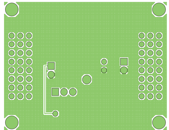
Figure 5: AAT4625 Evaluation Board Solder Side Layout.
