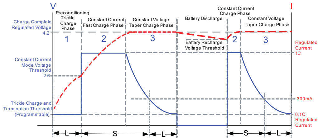
Figure 1: Current vs. Voltage and Charger Time Li-ion Battery Charging and Recharge Profile.
