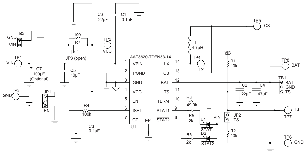
Figure 5: AAT3620 2A Evaluation Kit Schematic.
