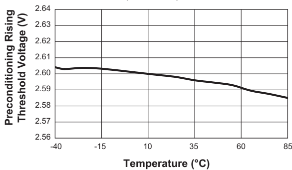
Preconditioning Rising Threshold Voltage vs. Temperature
