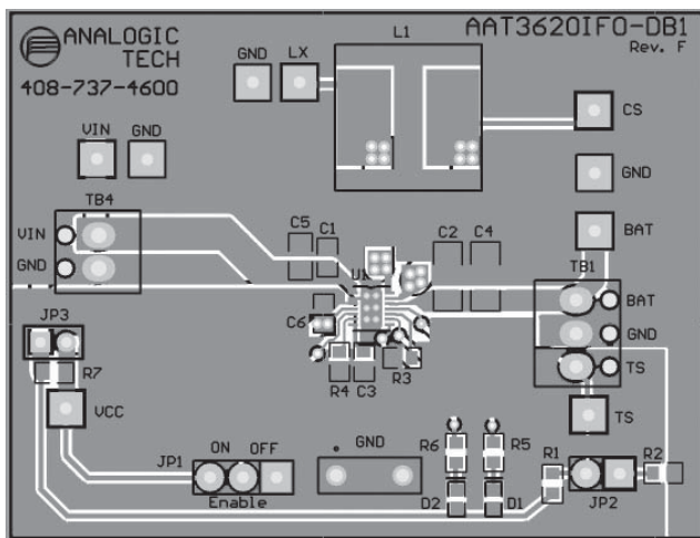
Figure 6: AAT3620 Evaluation Kit Top Layer.
