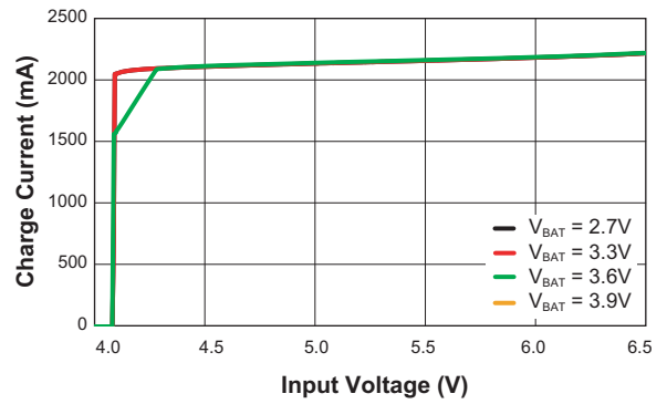
Charge Current vs. Input Voltage (T = 85°C)
