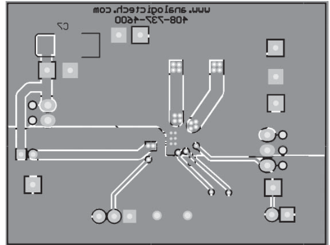
Figure 7: AAT3620 Evaluation Kit Bottom Layer.
