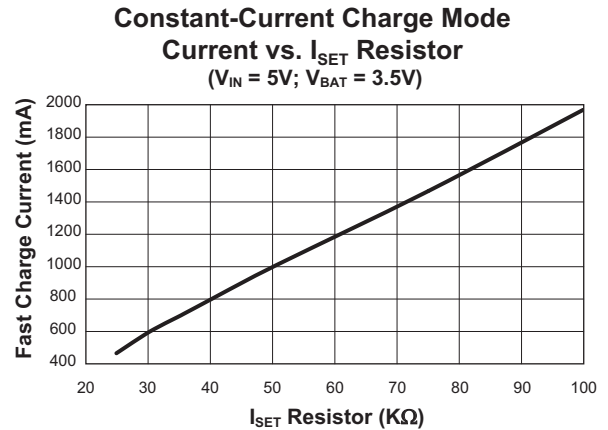
Figure 3: Constant-Current Mode Charge I_{CH\_CC} Setting vs. ISET Resistor.
