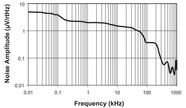
AAT3237 Self Noise
