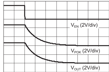
Time (200µs/div)
