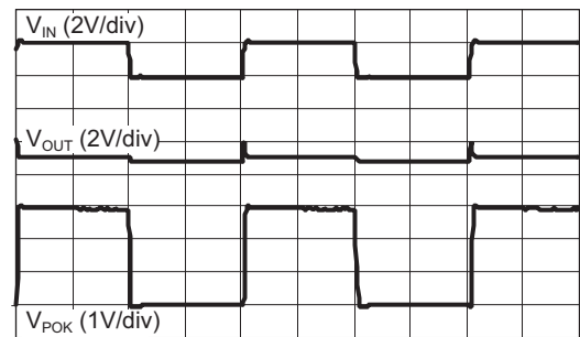
Time (200µs/div)
