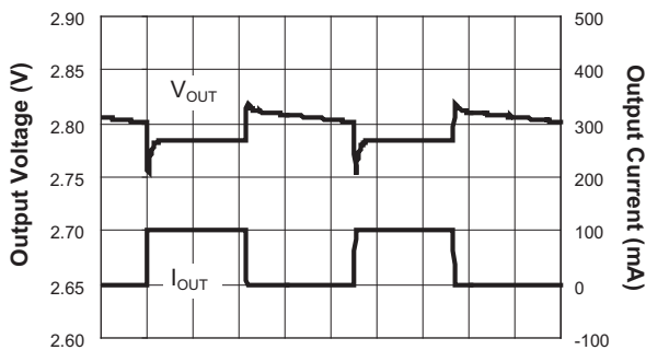
Time (100µs/div)
