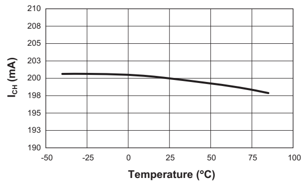
Constant Charging Current vs. Temperature (R SET = 8.06kΩ)
