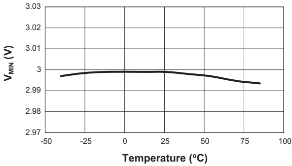
Preconditioning Threshold Voltage vs. Temperature (RSET = 8.06kΩ; AAT3684 Only)
