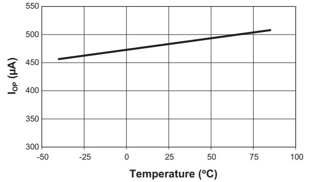
Operating Current vs. Temperature (RSET = 8.06kΩ)
