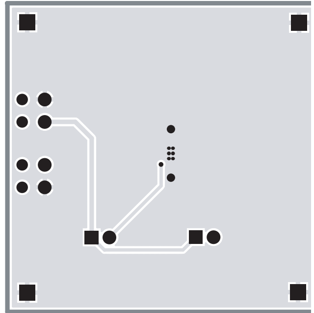
Figure 6: AAT3684 Evaluation Board Bottom Layer.
