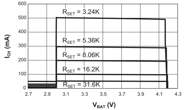
Charging Current vs. Battery Voltage (AAT3684 only)
