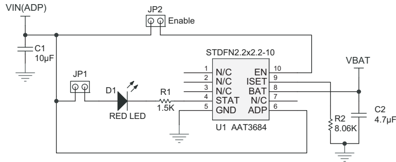
C1 10µF 10V 10% X5R 0805 GRM21BR61A106KE19 C2 4.7µF 6.3V 10% X5R 0603 GRM188R60J475KE19
