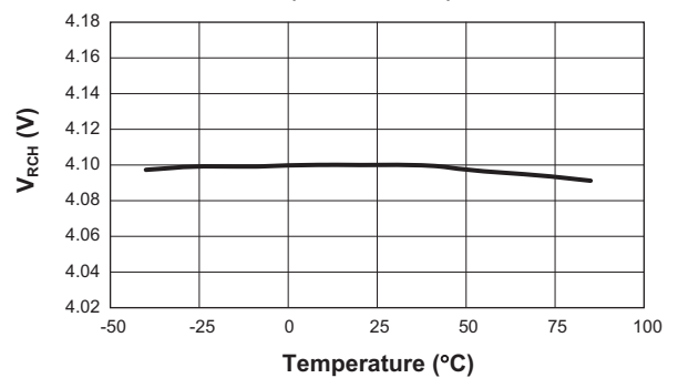
Recharging Threshold Voltage vs. Temperature (RSET = 8.06kΩ)
