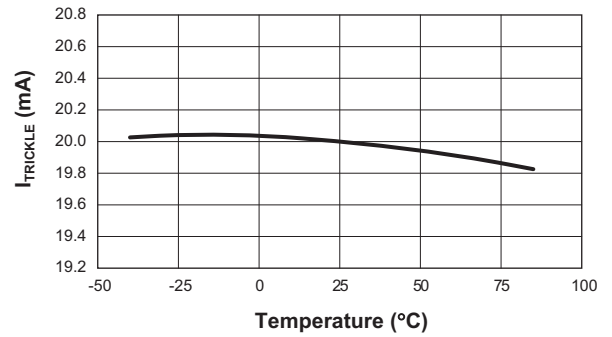
Preconditioning Charge Current vs. Temperature (RSET = 8.06kΩ; AAT3684 Only)
