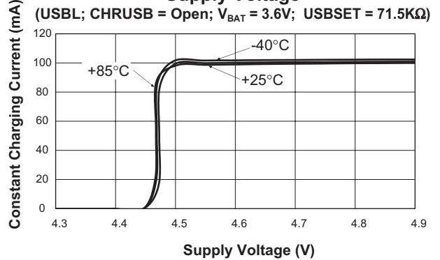
Constant Charging Current vs. Supply Voltage
