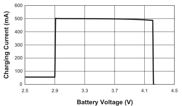
Charging Current vs. Battery Voltage (USBH; USBSET = 71.5KΩ)
