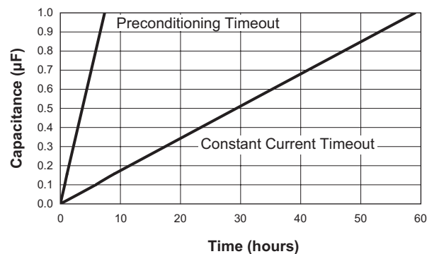
CT Pin Capacitance vs. Counter Timeout
