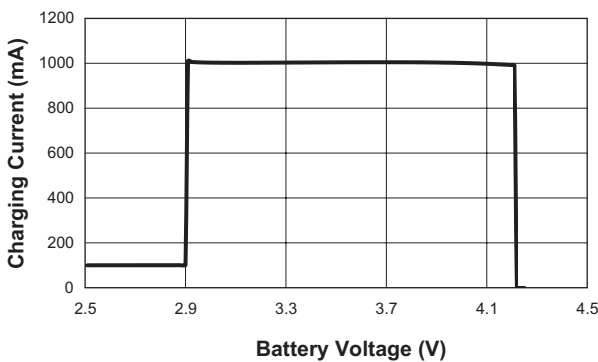
Charging Current vs. Battery Voltage (ADP; ADPSET = 57.6KΩ)
