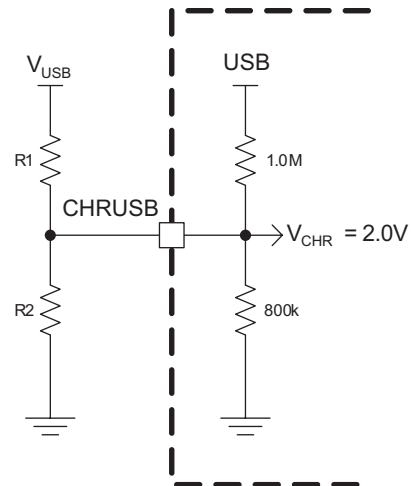
Figure 4: Internal Equivalent Circuit for the CHRUSB Pin.
