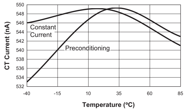
CT Current vs. Temperature ( C_T = 0.1F )
