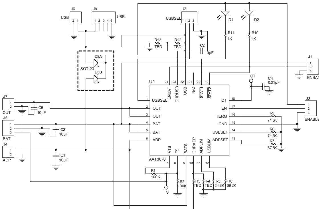
Figure 8: AAT3670 Evaluation Board Schematic.
