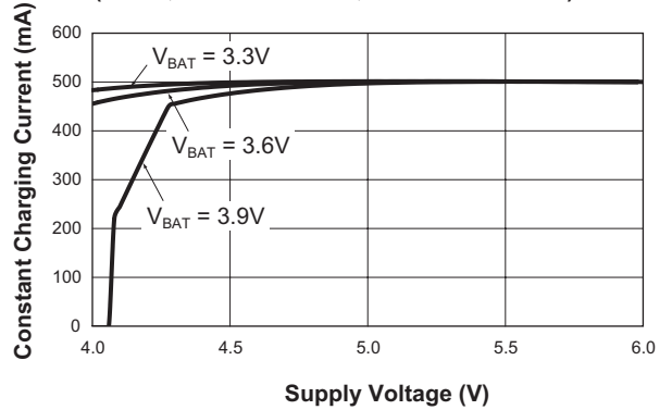
Constant Charging Current vs. Supply Voltage (USBH; CHRUSB = USB; USBSET = 71.5kΩ)
